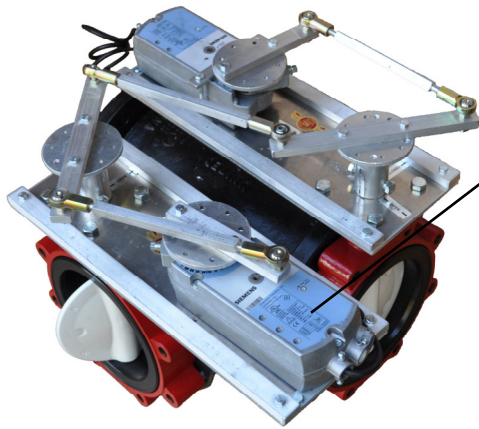
3-WAY VALVE ARRANGEMENTS
