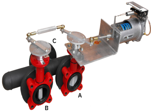
ASSEMBLY WITH Schneider Pneumatic ACTUATORS
