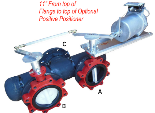
ASSEMBLY WITH Schneider PNEUMATIC ACTUATORS
